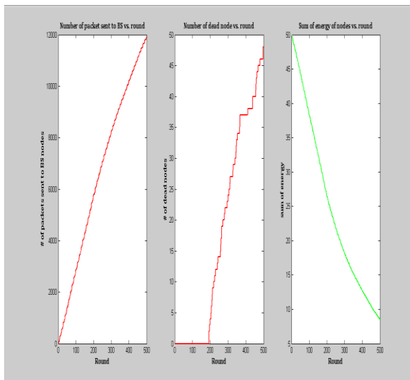
Fig 5.8 Simulations results for modified algorithms for 500 rounds
