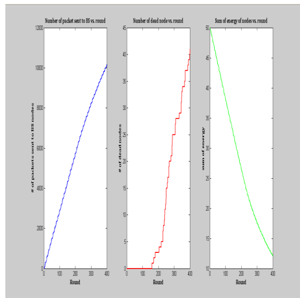
Fig 5.7 Simulations results for modified algorithms for 400 rounds
