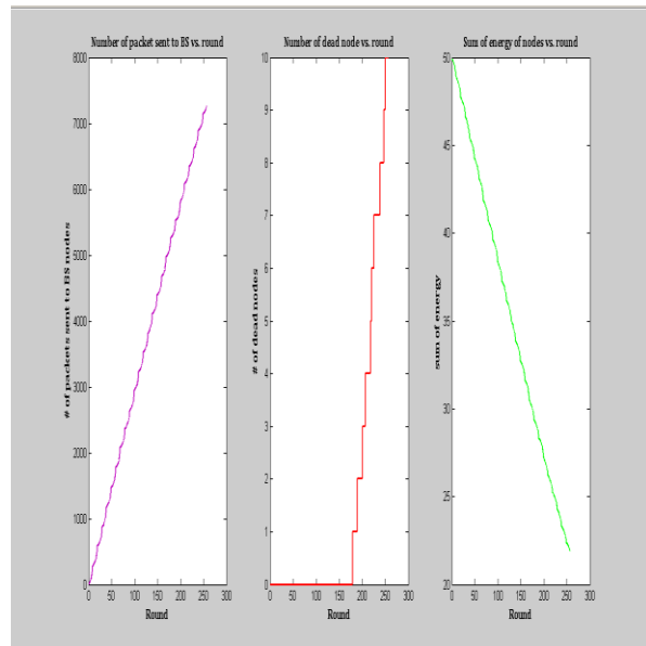
Fig 5.6 Simulations results for modified algorithms for 300 rounds
