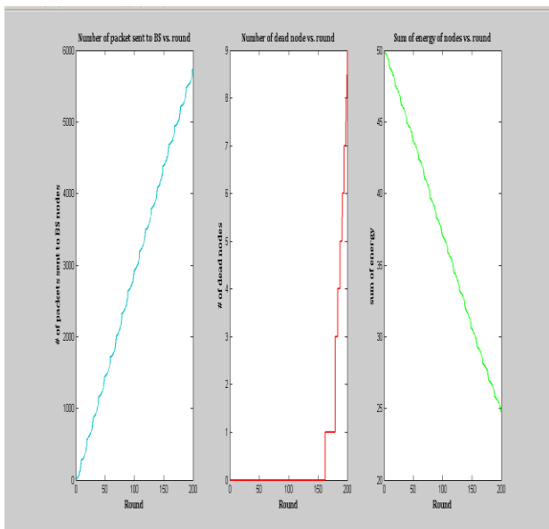
Fig 5.6 Simulations results for modified algorithms for 200 rounds
